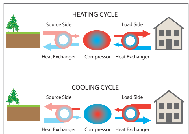
The three loops of the heating & cooling cycle
