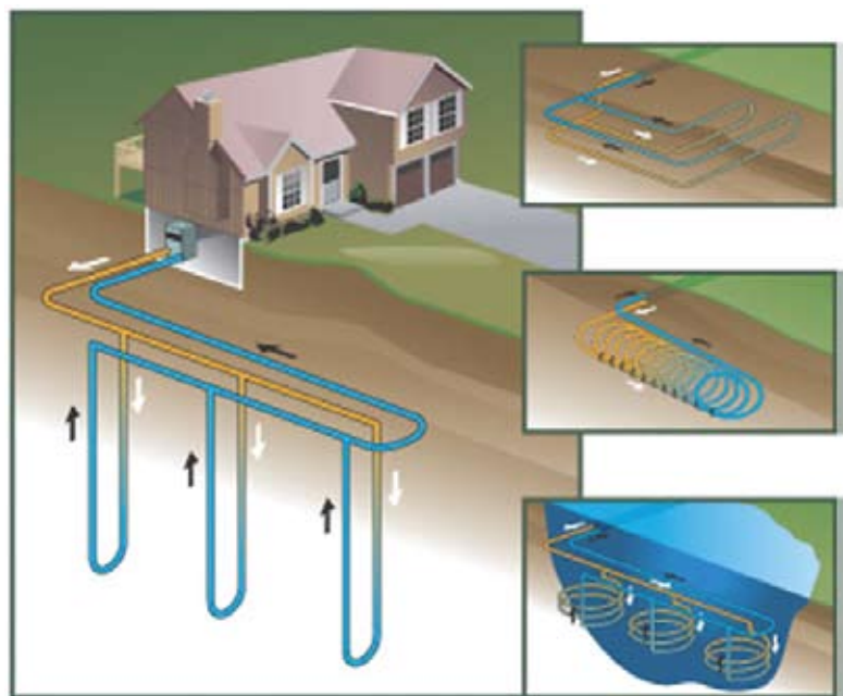
types of geothermal loops (clockwise from left) Vertical Loops, Horizontal loops, slinky loops and open loops.
