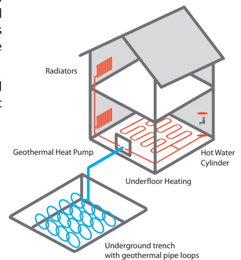
Layout of a typical geothermal heating system
